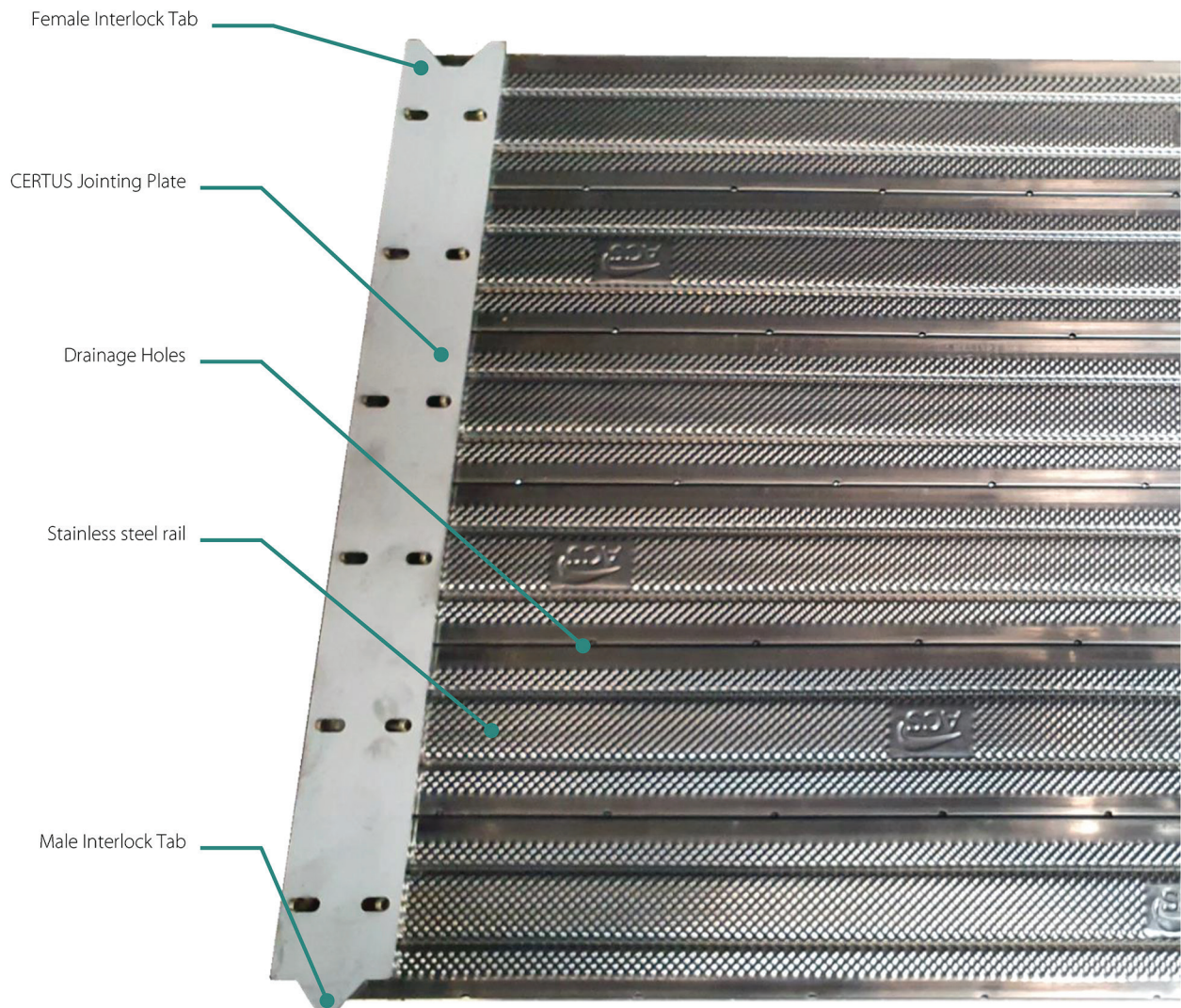
Rear Face of the ACS CERTUS Panel
