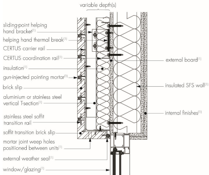
Window Head (option 4 – soffit section)
