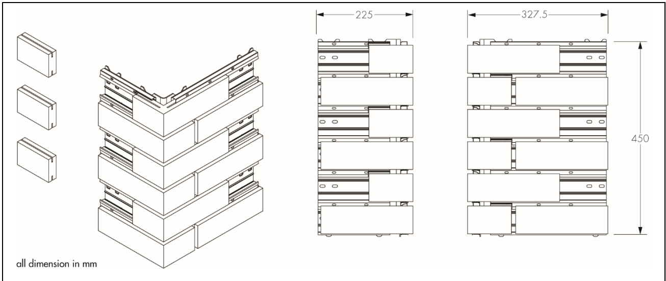
Figure 7 Standard 215 mm reveal
