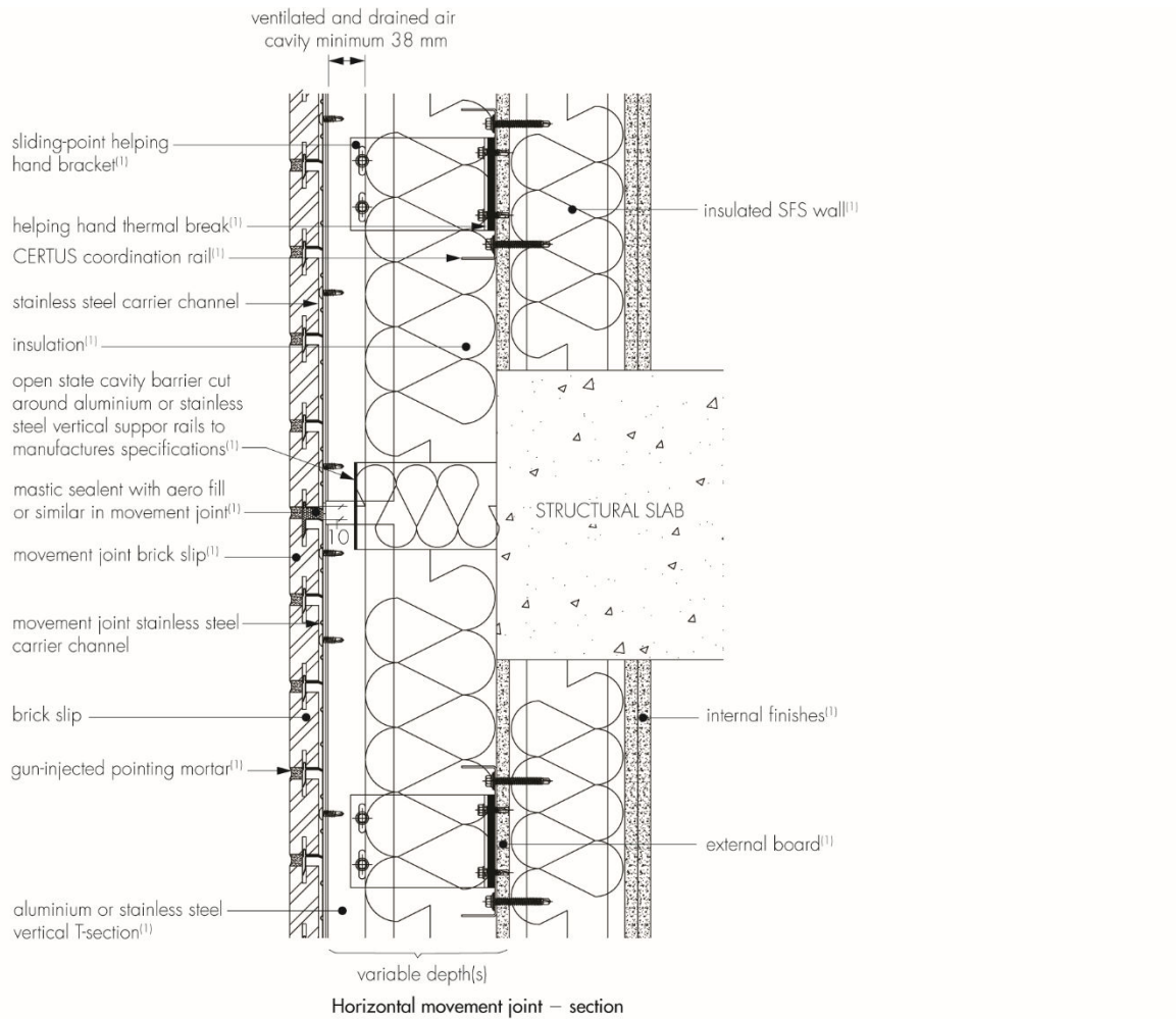
Figure 10 Horizontal and vertical movement joint
